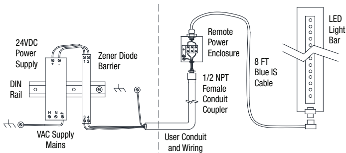
Non-Hazardous Area
